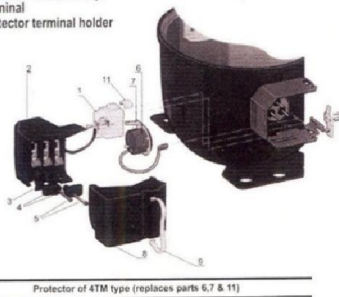
Protector of 4TM type (replaces parts 6,7 & 11)
